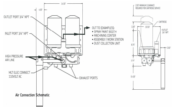
P/N 21999-0271 30 HP Dryer 135 SCFM
